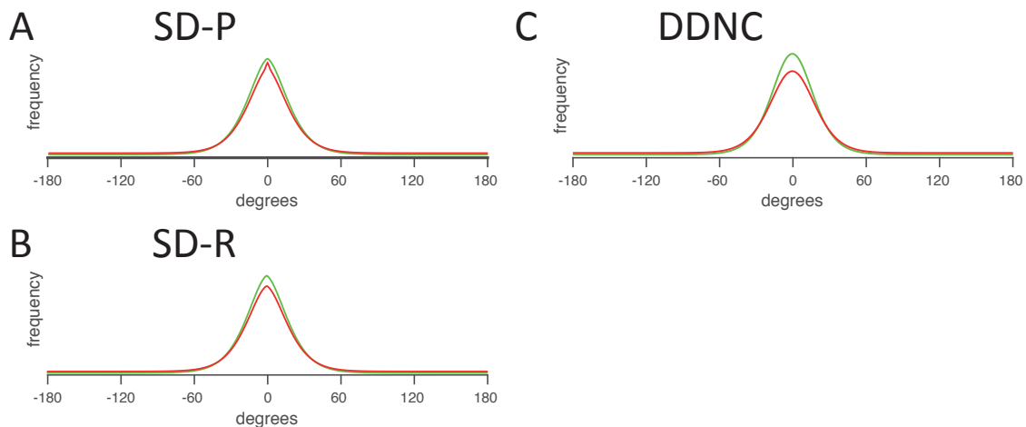
Figure 7: The model fitted distributions (using data from all participants) for short (green) and long (red) retention conditions for 3 models: Sudden Death-proportional (SD-P) (A), Sudden Death-random (SD-R) (B), and Degradation and Death by Natural Causes (DDNC) (C). Only the error distributions for the DDNC model (panel C) have more uncertainty during long retention (red), a characteristic found in the true data.
